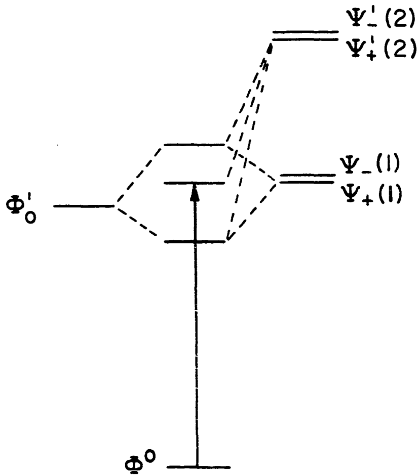
Figure 13. Energy diagram showing an ionized exciton transition \Psi_-(1) \leftarrow \Phi^0 . The interaction between the Frenkel exciton state \Phi^1 and \Psi_+(1) is also depicted
