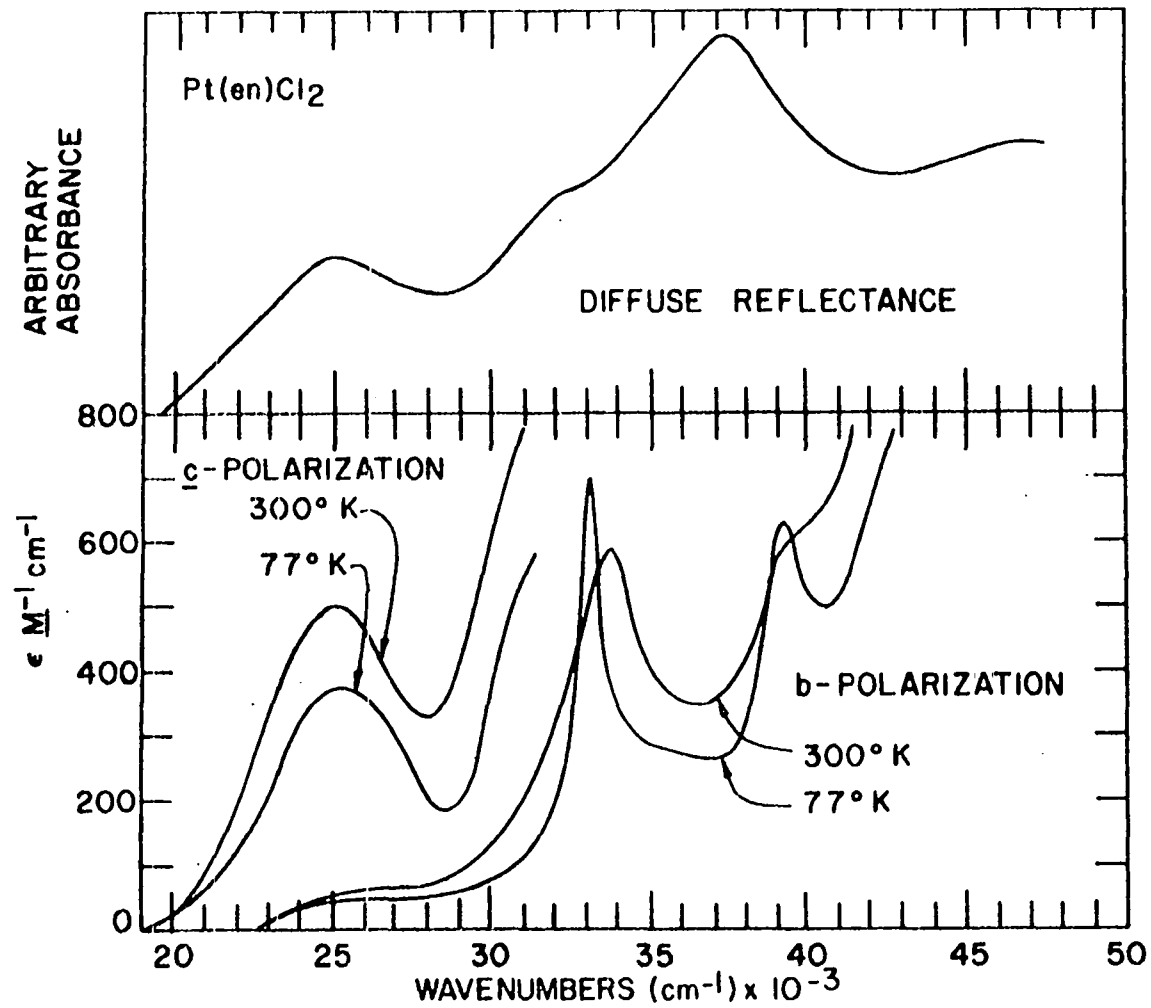
Figure 10. Diffuse reflectance spectrum and single crystal polarized absorption spectra for Pt(en)Cl 2
