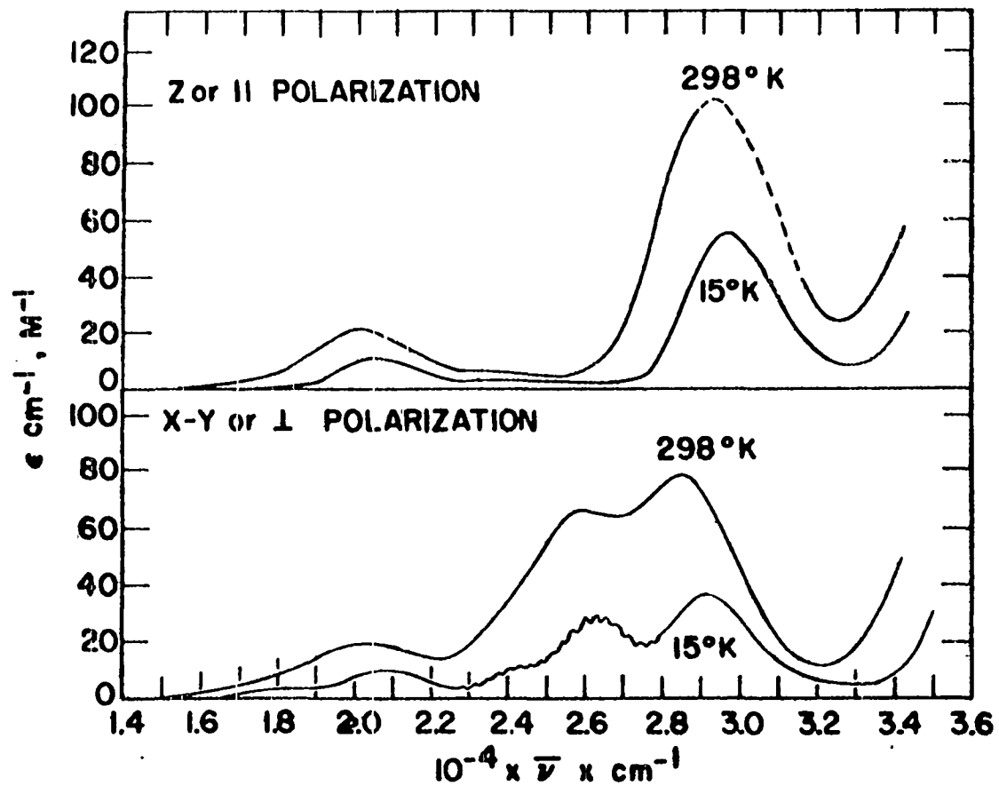
Figure 3. Polarized crystal spectra of K_2PtCl_4 at 298^\circ and 15^\circ K
