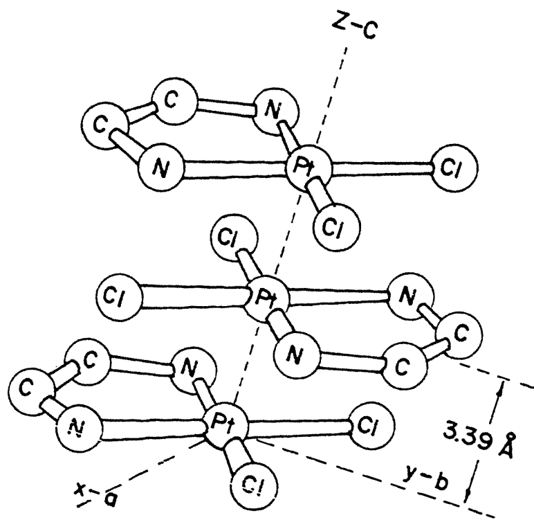
Figure 6. Stacking of the Pt(en)Cl 2 molecules along the c -direction
