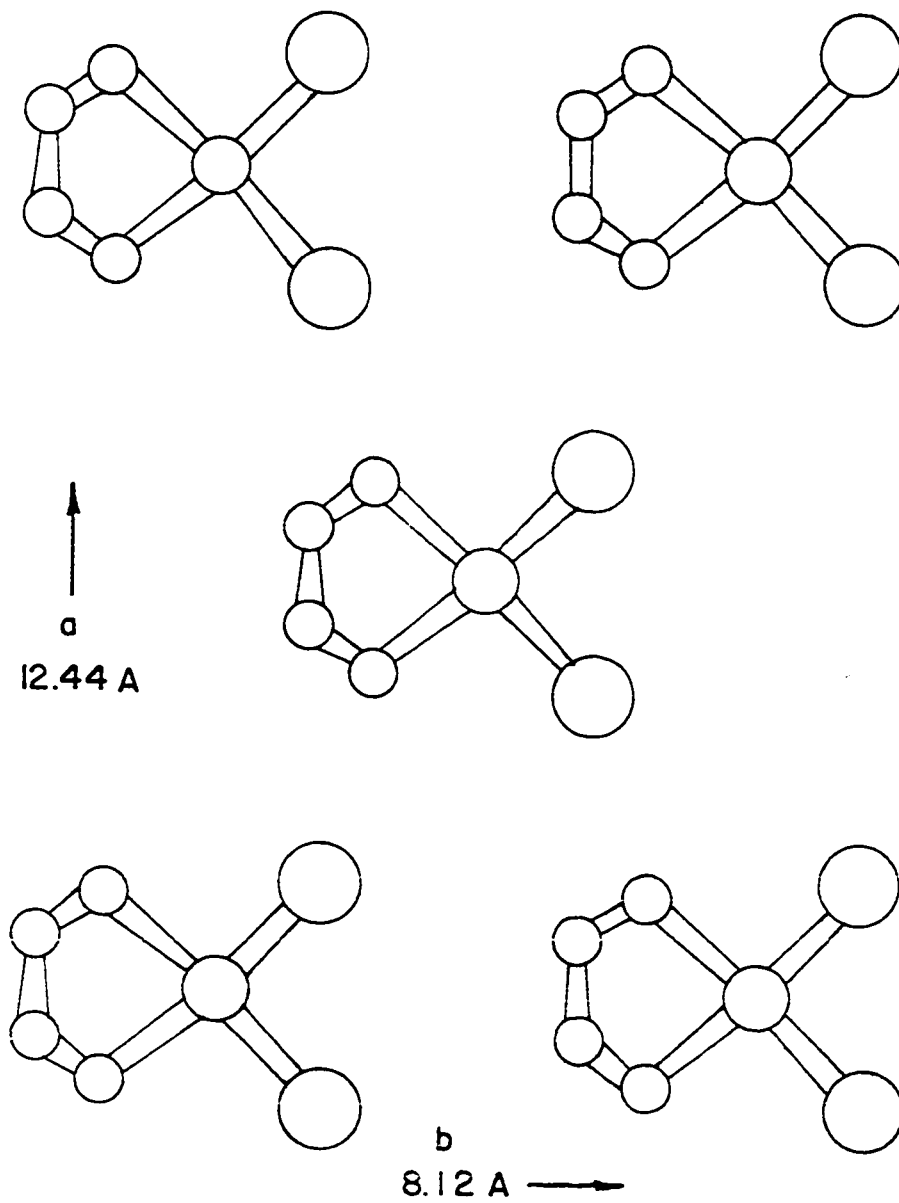
Figure 7. Orientation of Pt(en)Cl 2 molecules in an a-b plane
