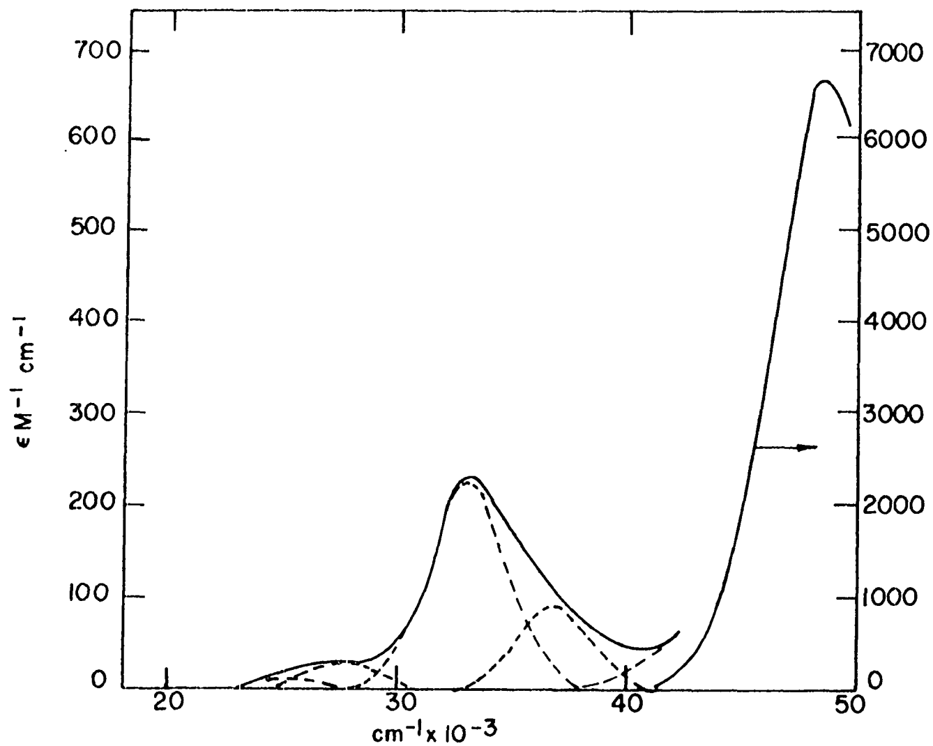
Figure 8. Solution spectrum of Pt(en)Cl 2 (solid lines). A Gaussian analysis is indicated by the dashed line
